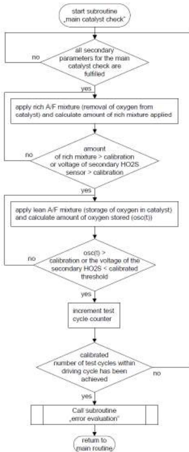
Figure 4: Aging monitoring of catalytic converters-main monitoring process subroutine
