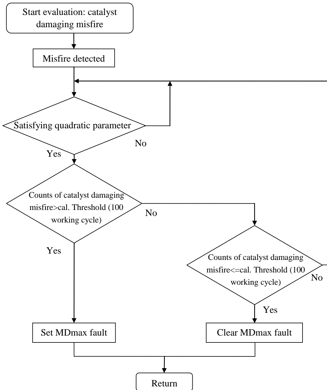
Figure 11: Misfire monitoring - subprogram "damage catalyst monitoring"
