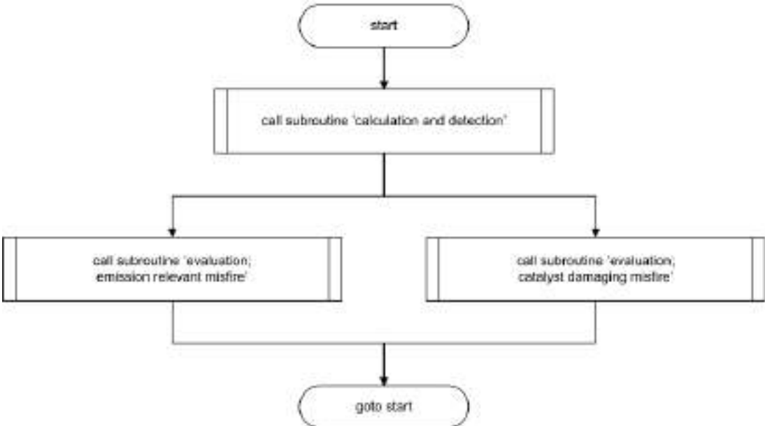
Figure 8: Misfire detection-main flowchart
