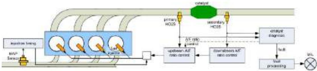
Figure 2: Catalytic converter aging monitoring system
