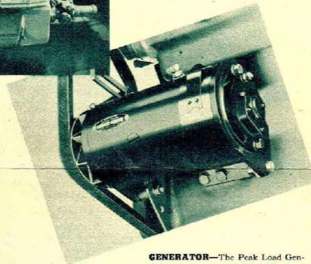
GENERATOR —The Peak Load Generator used on the 1936 La Salle is an ingenious device that keeps the battery fully charged and compensates, automatically, for the output demanded by radio, heater, lights, and other electrically-operated equipment.
