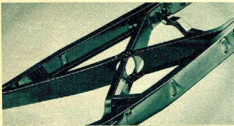
FRAMES —Frame of the new La Salle is of the X type, riveted and welded together into a single unit, and so strongly built it resists effectively strain and stress. Literally, a frame within a frame of bridge-like construction.
