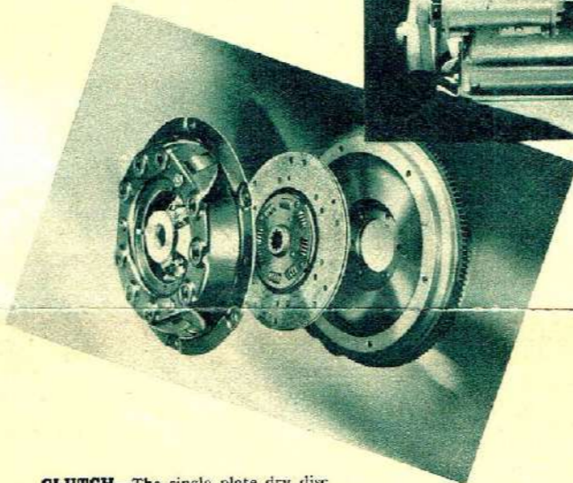
CLUTCH —The single plate dry disc type La Salle clutch has facings made of a long wearing fabric that resists heat and gives smooth operation. Clutch facing area is 10 inches outside diameter and 6 inches inside diameter.
