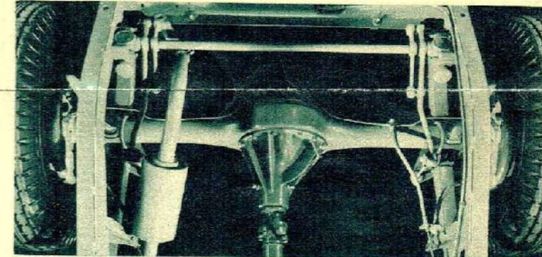
STABILIZERS —One of the many remarkable safety and comfort advantages in the new La Salle is the Ride Stabilizer—eliminates dangerous sidesway—keeps the car on an even keel rounding curves and corners.
