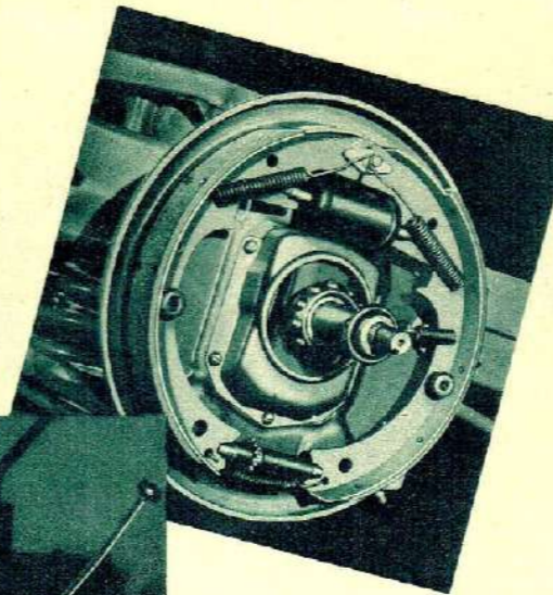
BRAKES —La Salle is equipped with improved Super-Hydraulic Brakes with new centrifuse brake drums, providing equalized braking on all four wheels an essential to confidence and ease of mind under all driving conditions.
