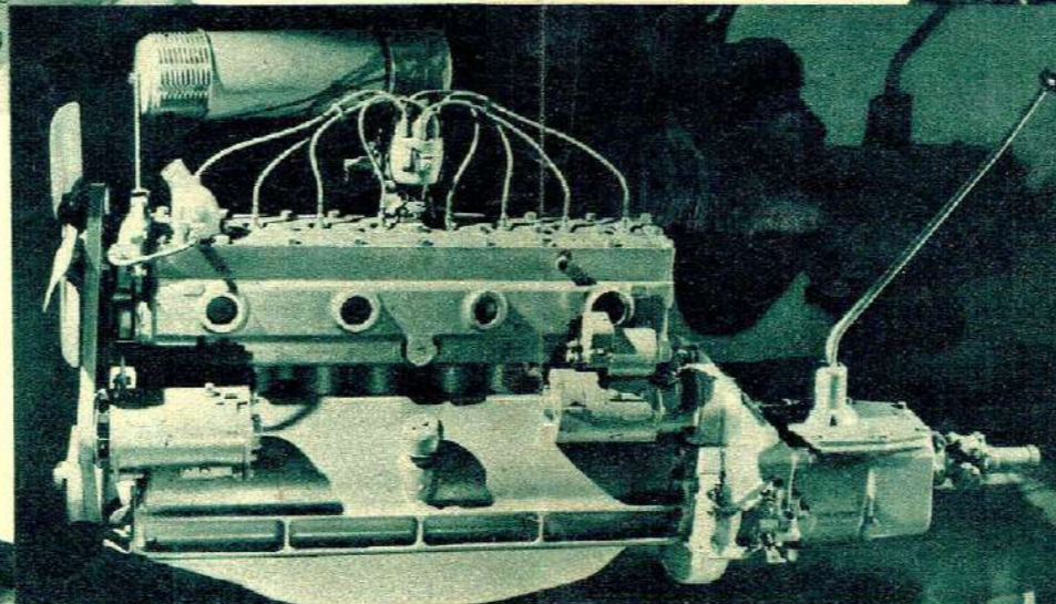
MOTOR —The engine in the new La Salle is of the straight eight type, incorporating the latest in engineering and manufacturing developments. Unbelievably smooth, economical, long-lived, the La Salle engine is the kind of power plant you would expect Cadillac to build—fully counter-weighted crankshaft, anodized aluminum alloy pistons—honed-in cylinder bores—exclusive manifold design for greater power and performance, and many other valued features.
