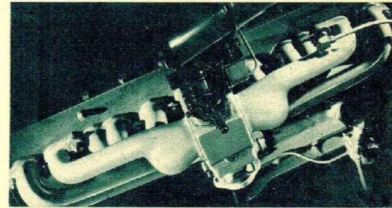
MANIFOLDING —Perfect performance can be achieved only with perfect and equal fuel distribution. The La Salle Equalized Manifolding System brings the carburetor equi-distant to each cylinder, exacts the utmost energy from each of the eight cylinders and each drop of fuel.
