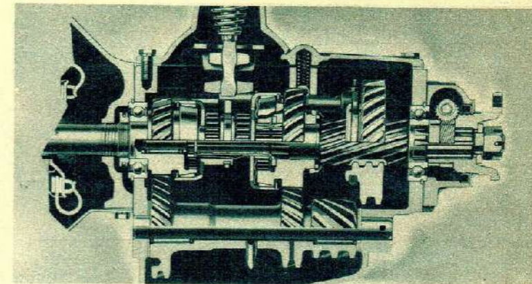
TRANSMISSION —The famous Cadillac-pioneered Synco-Mesh Transmission, greatly improved and even more quiet, is used in the La Salle for 1936. Result—swifter, surer shifting—no clash at any speed—safe control on hills and slippery roads—more enjoyable to drive.
