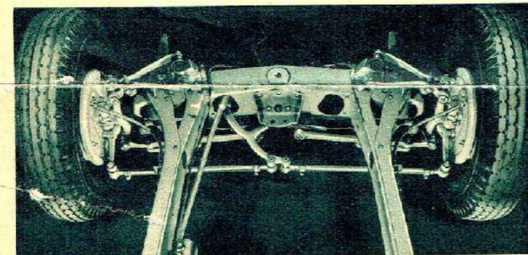
STEERING —The new La Salls embody the latest development in steering—Center Point Steering—made possible by Knee-Action wheels—and providing unusual sureness and safety. This construction insulates the steering wheel against road shocks—when turning or rounding corners, wheel returns, of itself, to straight-ahead position.
