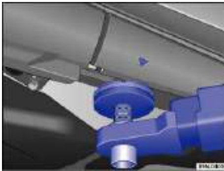
Fig. 176 Rear lift point for workshop hoist or floor jack.
