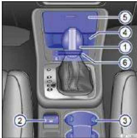
Fig. 8 Vehicles without Keyless Access: Overview of center console lower section.
