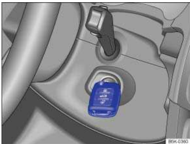
Fig. 127 Emergency starting feature on vehicles with Keyless Access.
