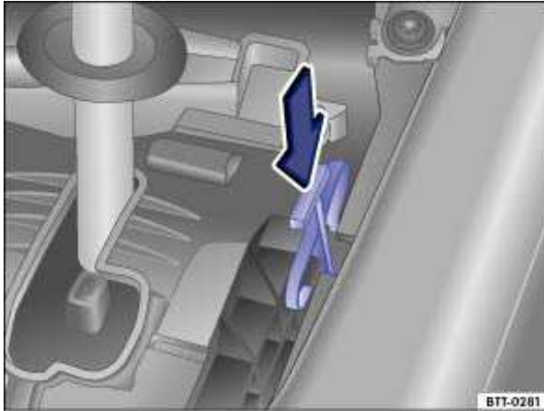
Fig. 178 Releasing the selector lever lock.
