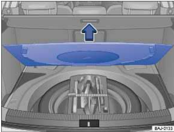
Fig. 180 In the luggage compartment: Spare wheel and vehicle tool kit
