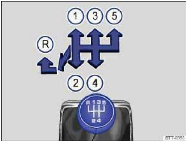
Fig. 131 Gearshift pattern of a 5-speed manual transmission.
