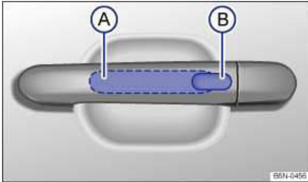
Fig. 27 Keyless Access locking and starting system: Sensor for unlocking A on the inside of the front door handles. Sensor for locking B on the outside of the front door handles.
