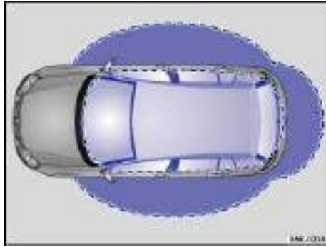
Fig. 24 Ranges of the Keyless Access system. Outside the vehicle: Unlocking range. Inside the vehicle: Starting range.
