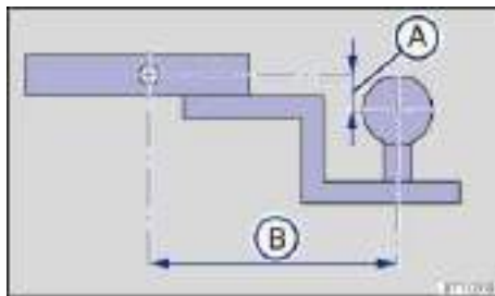
Fig. 101 Dimensions of the ball mount support.
