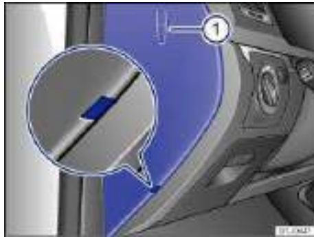
Fig. 188 On the driver side in the instrument panel: Fuse box cover with plastic tweezers 1 on the inside of the cover.
