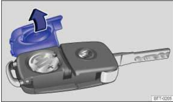
Fig. 19 Remote control vehicle key: Open battery compartment cover.
