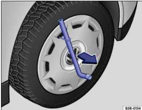
Fig. 139 Pulling the wheel cover off (Version 1).
