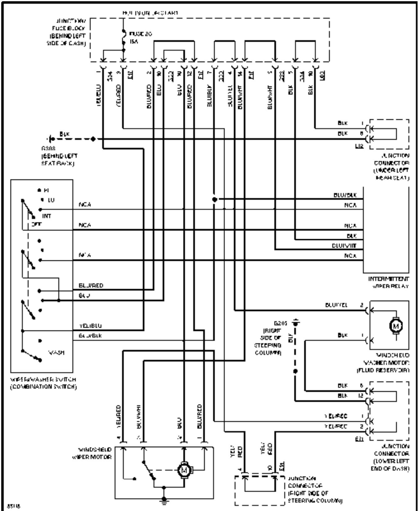
Wiper/Washer Circuit
