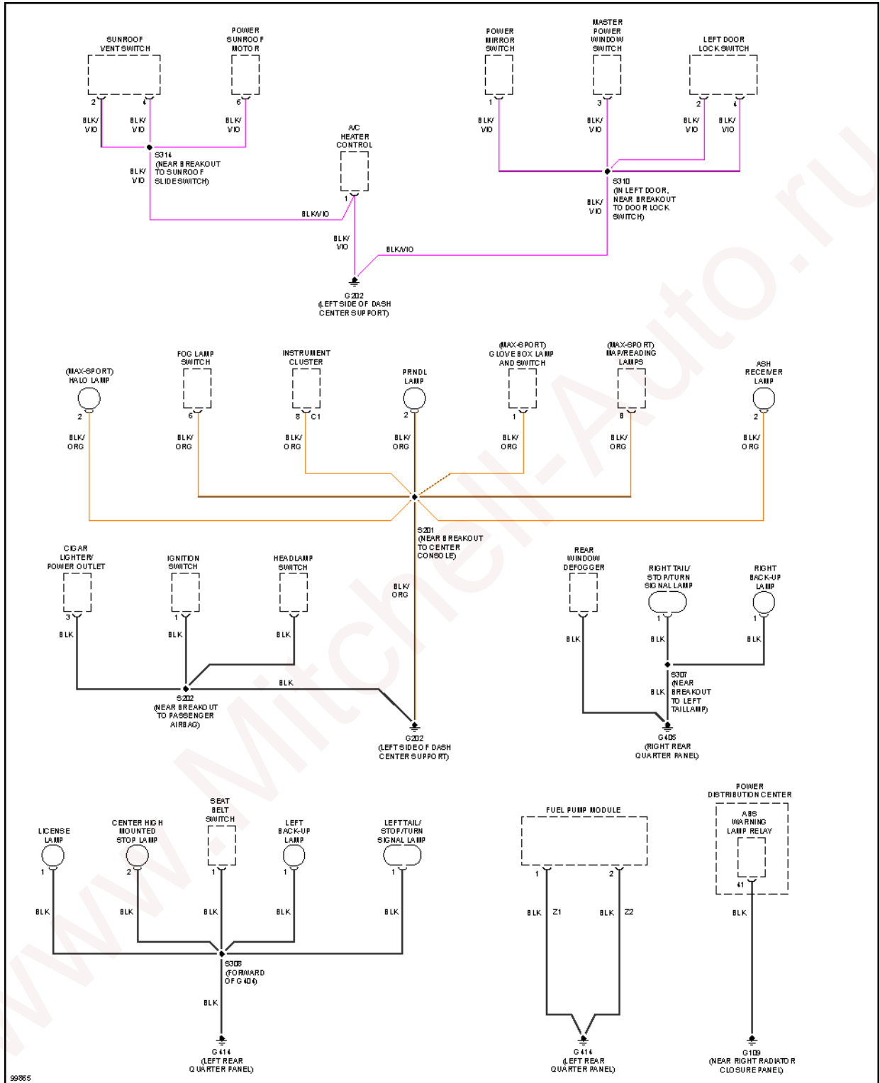
Fig. 14: Ground Distribution Circuit (2 of 2)
