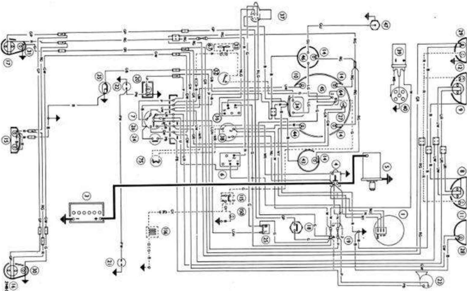
Mini 1000 Special De-luxe Saloon (with alternator and rocker type switches)
