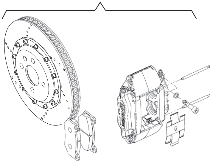
Big Brake Kit (sport) 2 piece disc without adaptor
