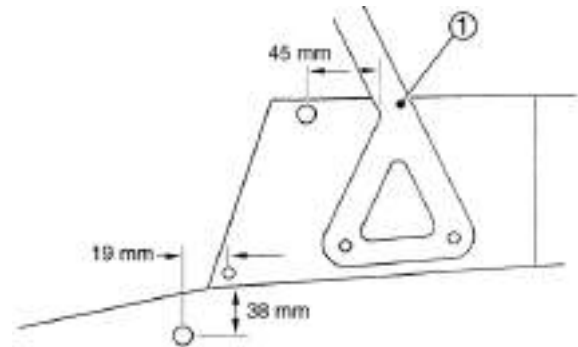
Figure 170: Tonneau cover fasteners (front)
