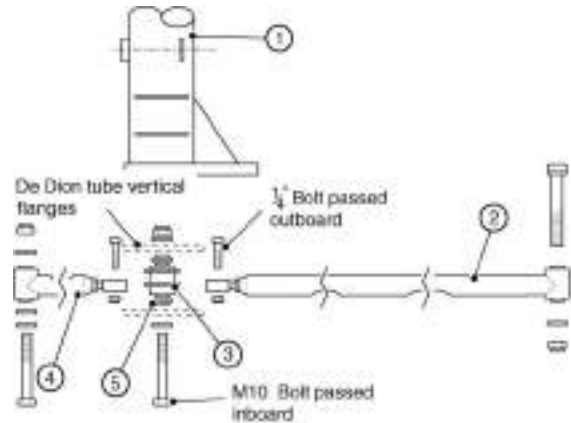
Figure 127: Watts link - RH top view
