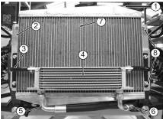
Figure 108: Radiator arrangement
