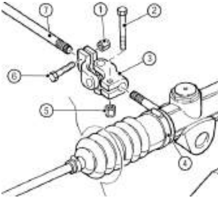
Figure 28: Steering rack to steering column
