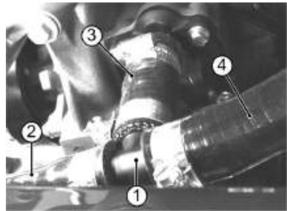
Figure 85: Coolant hoses
