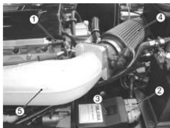
Figure 96: ECU
