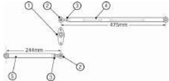
Figure 126: Watts link - RH side
