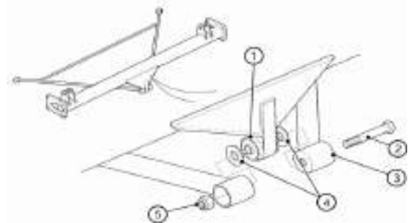
Figure 129: Metalistic brush - De Dion tube
