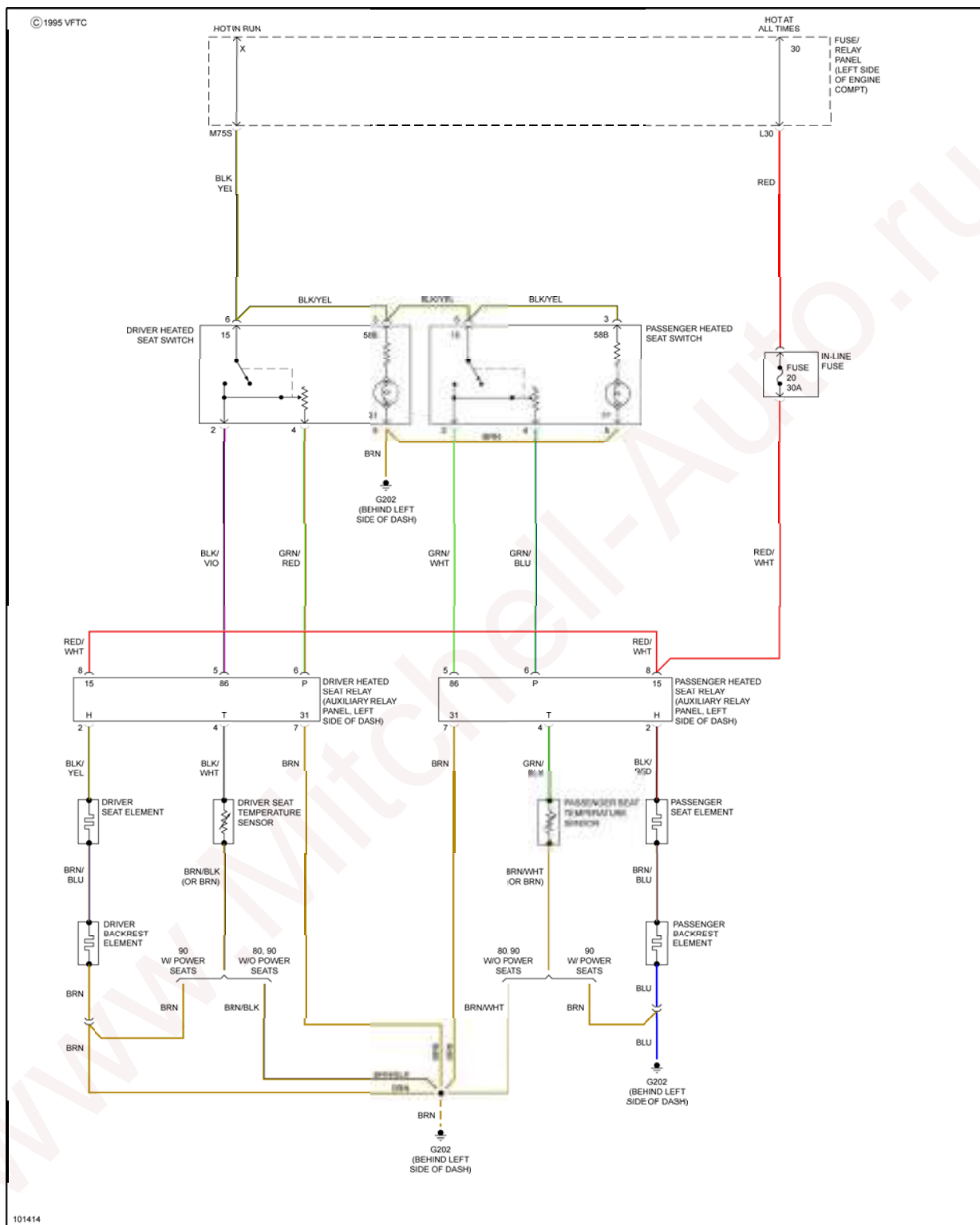
Fig. 10: Heated Seats Circuit
