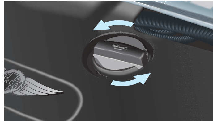
Oil Filler Cap located under the right bonnet.
